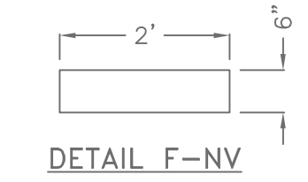
DETAIL F-NV 1600 UNIT UNVENTED CUPOLA FASCIA COMPONENT DETAIL (18 PIECES OF EACH REQUIRED) SCALE: 1/2"=1'-0"
