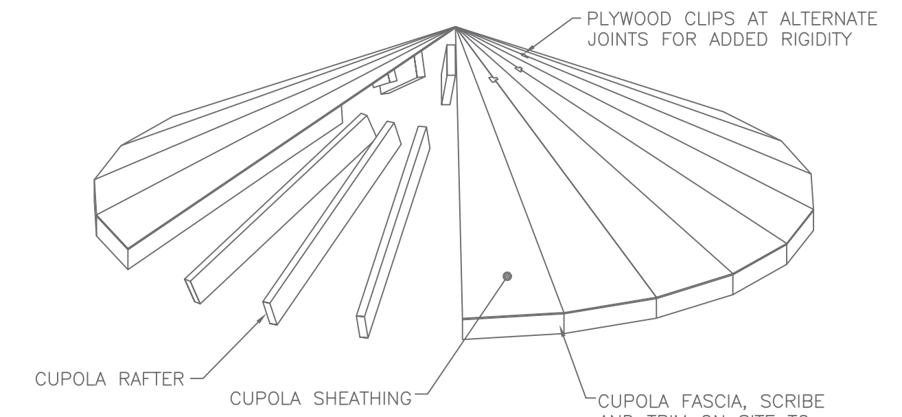
DETAIL D-NV UNVENTED CUPOLA ILLUSTRATION SCALE: NTS
