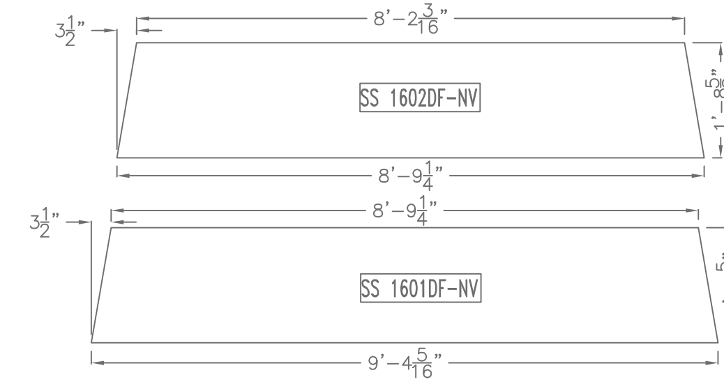
DETAIL D3-NV 1600 3'-9" OH HARDI SOFFIT SHEATHING DETAIL (UNVENTED WITH FOAM) 18 OF EA. REQUIRED
