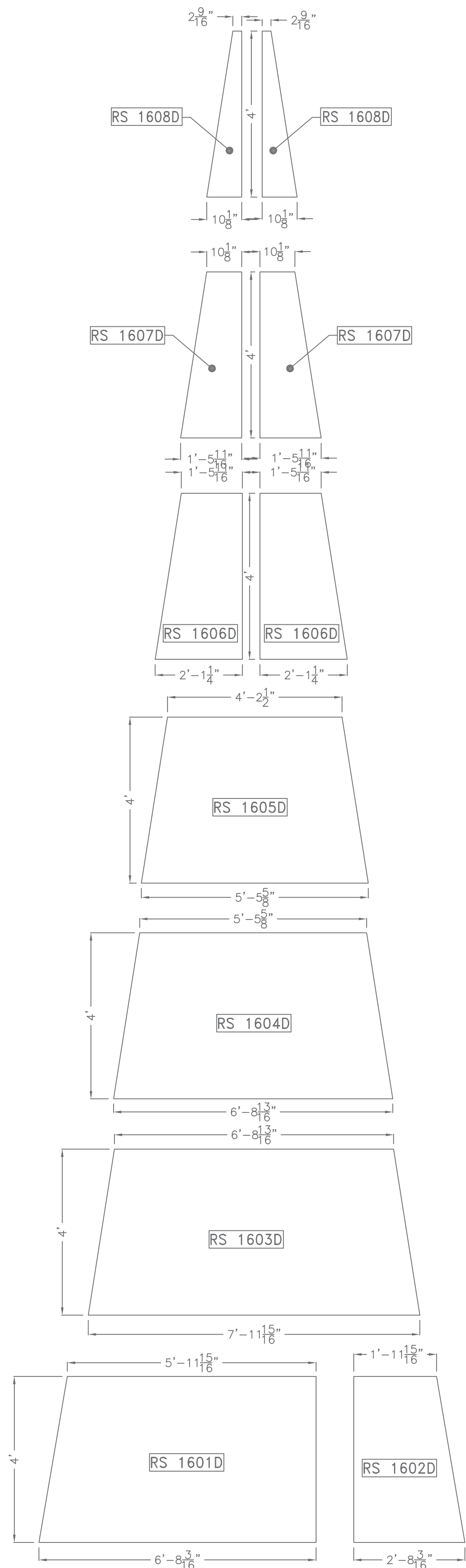
DETAIL B 1600 UNIT 3'-9" OVERHANG ROOF SHEATHING COMPONENT DETAIL SHEATHING MATERIAL: 5/8" CDX PLYWOOD (18 PIECES OF EACH REQUIRED) SCALE: 1/2"=1'-0"
