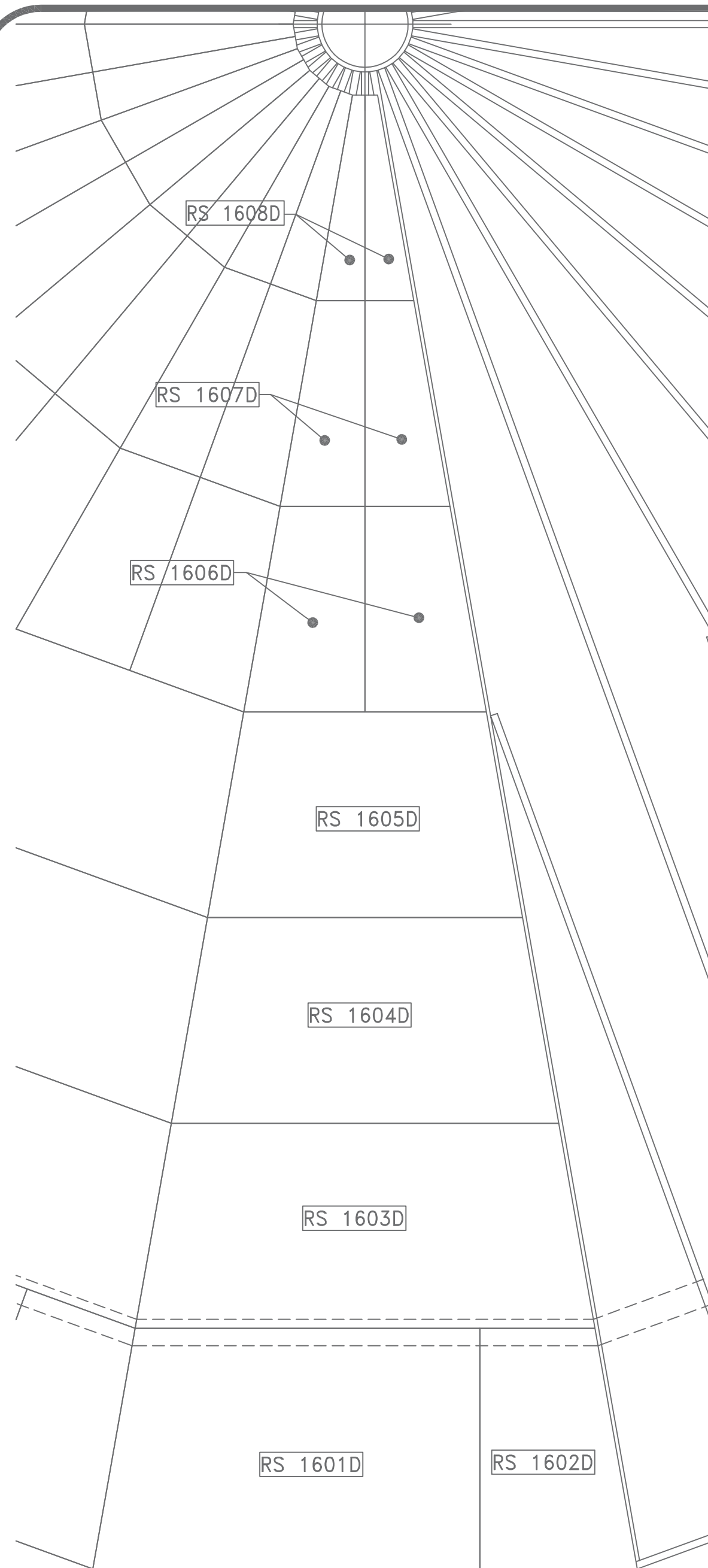
DETAIL A 1600 UNIT 3'-9" OVERHANG ROOF SHEATHING PLACEMENT DETAIL SHEATHING MATERIAL: 5/8" CDX PLYWOOD (18 PIECES OF EACH REQUIRED) SCALE: 1/2"=1'-0"
