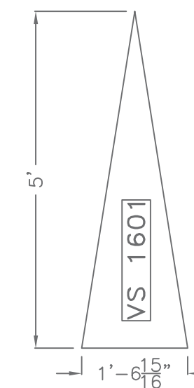
DETAIL E 1600 UNIT CUPOLA SHEATHING COMPONENT DETAIL SHEATHING MATERIAL: 5/8" CDX PLYWOOD (18 PIECES OF EACH REQUIRED) SCALE: 1/2"=1'-0"
